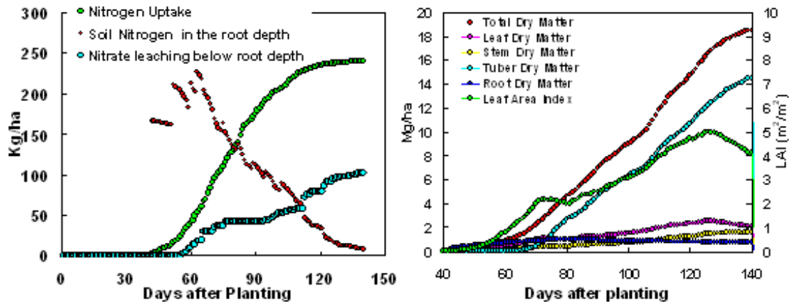
Figure 2. Predicted nitrogen uptake, soil nitrogen in the root depth and nitrate leaching below the root depth. (Example: 2001 data for 112 Kg/ha pre-plant N treatment (left) and predicted dry Matter and leaf area index (Example: 2001 data for 112 Kg/ha pre plant N treatment) (right).
