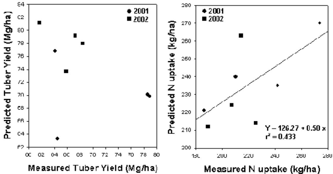
Figure 1. Comparison of predicted vs measured tuber yields and N uptake.
