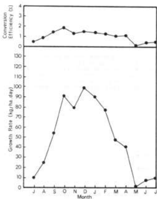
Figure 1. Growth rate and percent conversion of solar energy to plant DM of a paspalum dominant pasture in northern Victoria (From 8). The average yield of this pasture over five years was 18.3 t DM/ha - 50% greater than the regional average.
