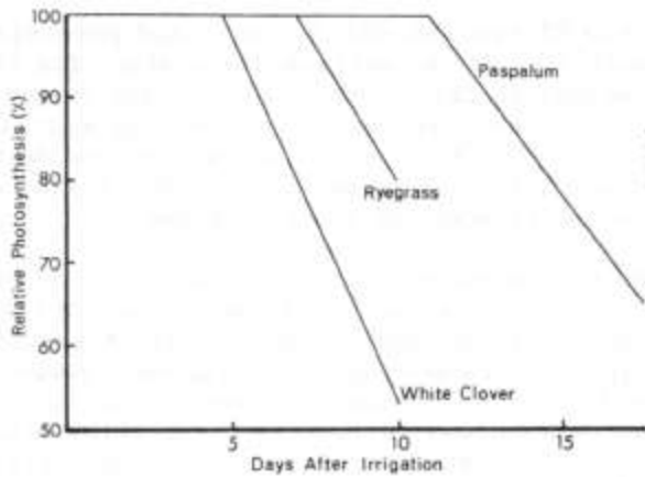
Figure 5. Photosynthetic rates (% of a well watered control) for pure swards of paspalum, perennial ryegrass and white clover during a drying cycle after irrigation (From 22).
