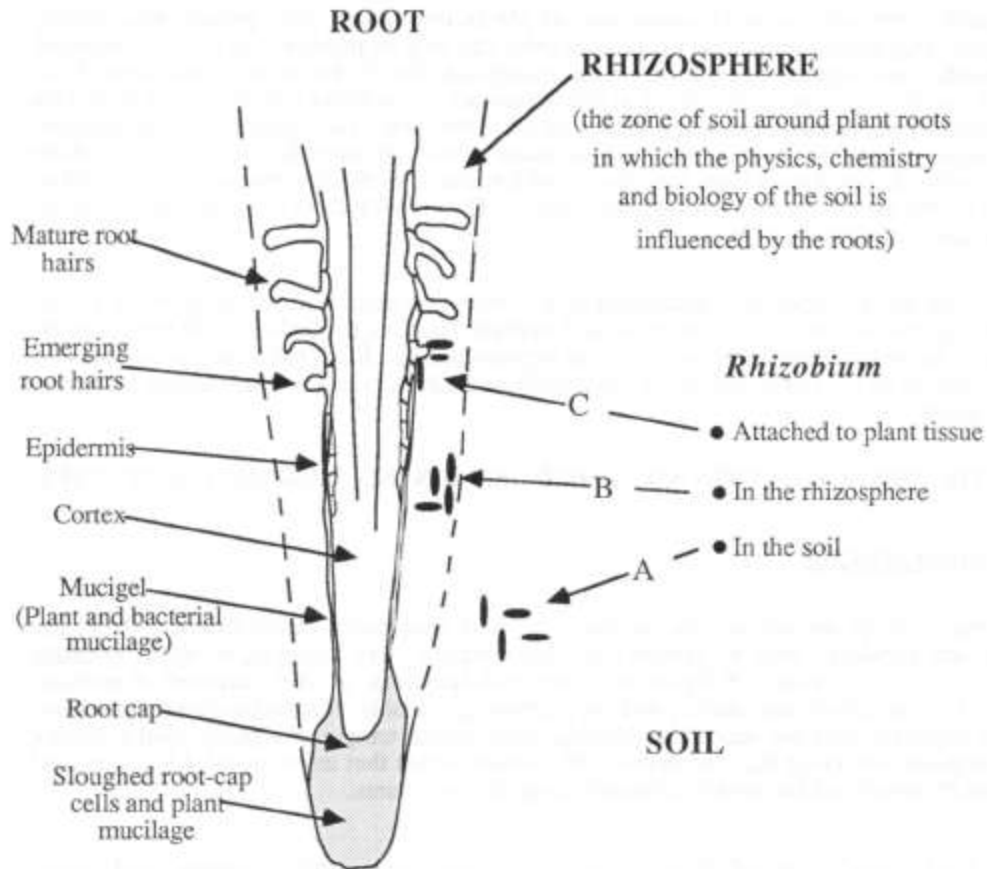
Figure 2. Diagram of a typical legume root. Rhizobia exist either as; saphrophytes in the soil and rhizosphere or as parasites on the root surface before becoming symbionts within the plant tissue.
